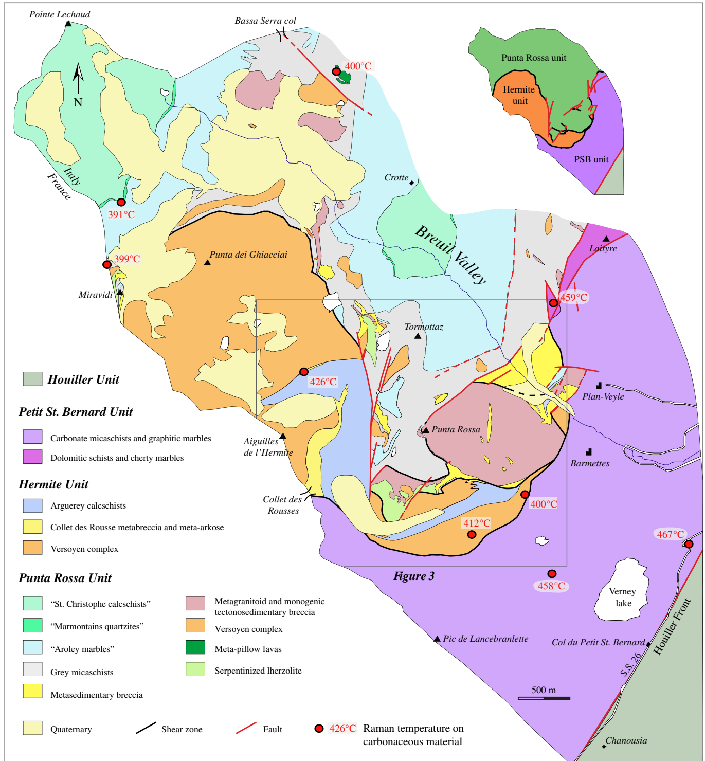
Fig. 2. Simplified geological map of the Valaisan units in the Breuil Valley. Red dots indicate sampling localities for Raman analyses on carbonaceous material. Inset shows the different tectonostratigraphic units detected in the area.
