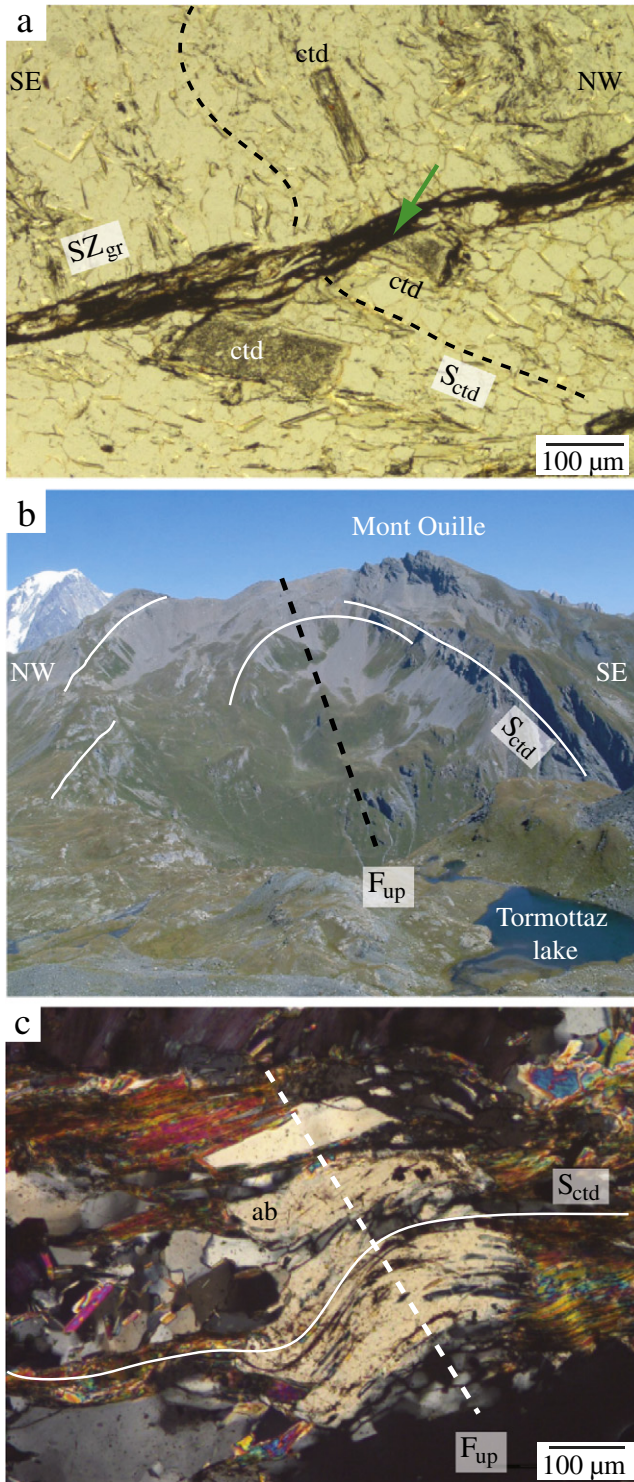
Fig. 8. Structural elements of the Punta Rossa unit. (a) Metamorphic fabrics related to SZ_{gr} dissect and dismember chlorite + white mica aggregates developed at the expense of former chloritoid elongated along S_{ctd} (green arrow). This observation indicates that shearing post-dated retrogression of ctd under greenschist facies conditions; (b) large scale upright fold ( F_{up} ) on the north-eastern side of the Breuil Valley; (c) F_{up} fold hinges are statically overgrown by albite porphyroblasts.
