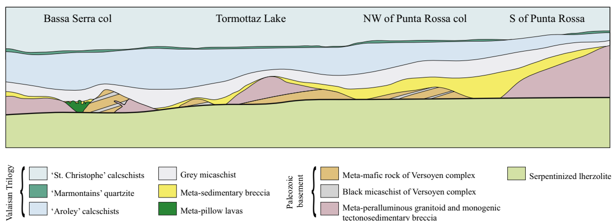
Fig. 12. Reconstruction of the pre-Alpine architecture of the Punta Rossa unit, showing windows of exhumed mantle between Paleozoic basement allochthons. Submarine lava flows are rare. The areas where the depicted lithostratigraphic associations can be observed are indicated.
