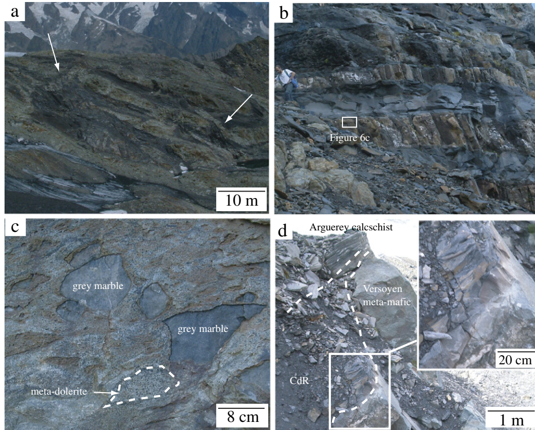
Fig. 6. Lithostratigraphy of the Hermite unit: (a) multiple generations of cross cutting metamafic layers in the Versoyen complex. Arrows indicate the youngest dykes. (b) Outcrop of Collet des Rousses metabreccia, with darker layers consisting mainly of prasinitic meta-arkose and green-brownish layers consisting of polymictic breccia with clasts of gray marble and metamafics analogous to the Versoyen complex (c); (d) contact between Versoyen complex metamafics, Collet des Rousses metabreccia and Arguerey calcschists. Inset shows clasts in Collet des Rousses metabreccia. Outcrop location is indicated in Fig. 11b.
