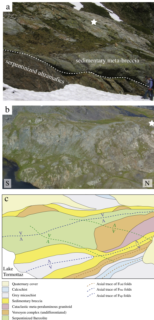
Fig. 4. Relationship between serpentinitized ultramafics, Paleozoic basement and Mesozoic metasediments in the Punta Rossa unit. On the ridge to the SW of Punta Rossa, serpentinitized ultramafics are locally overlain by polymictic breccias of sedimentary origin (a). Note that the tremolite-rich fabric in the ultramafics in the center of the picture is truncated by the lithological contact with the breccia, suggesting minor reactivation. Star marks the location of the outcrop shown in Fig. 5i. In the Tormottaz lake area (b) ultramafics crop out in the core of a F_{rec} synform (see Section 4 for explanation) and are directly in contacts with slivers of cataclastically deformed peraluminous metagranitoids and metamafics. All the above lithologies are overlain by a polymictic breccia and by radiolaria-bearing gray micaschists. Star marks the location of the metamorphic fault breccia shown in Fig. 5d and e.
