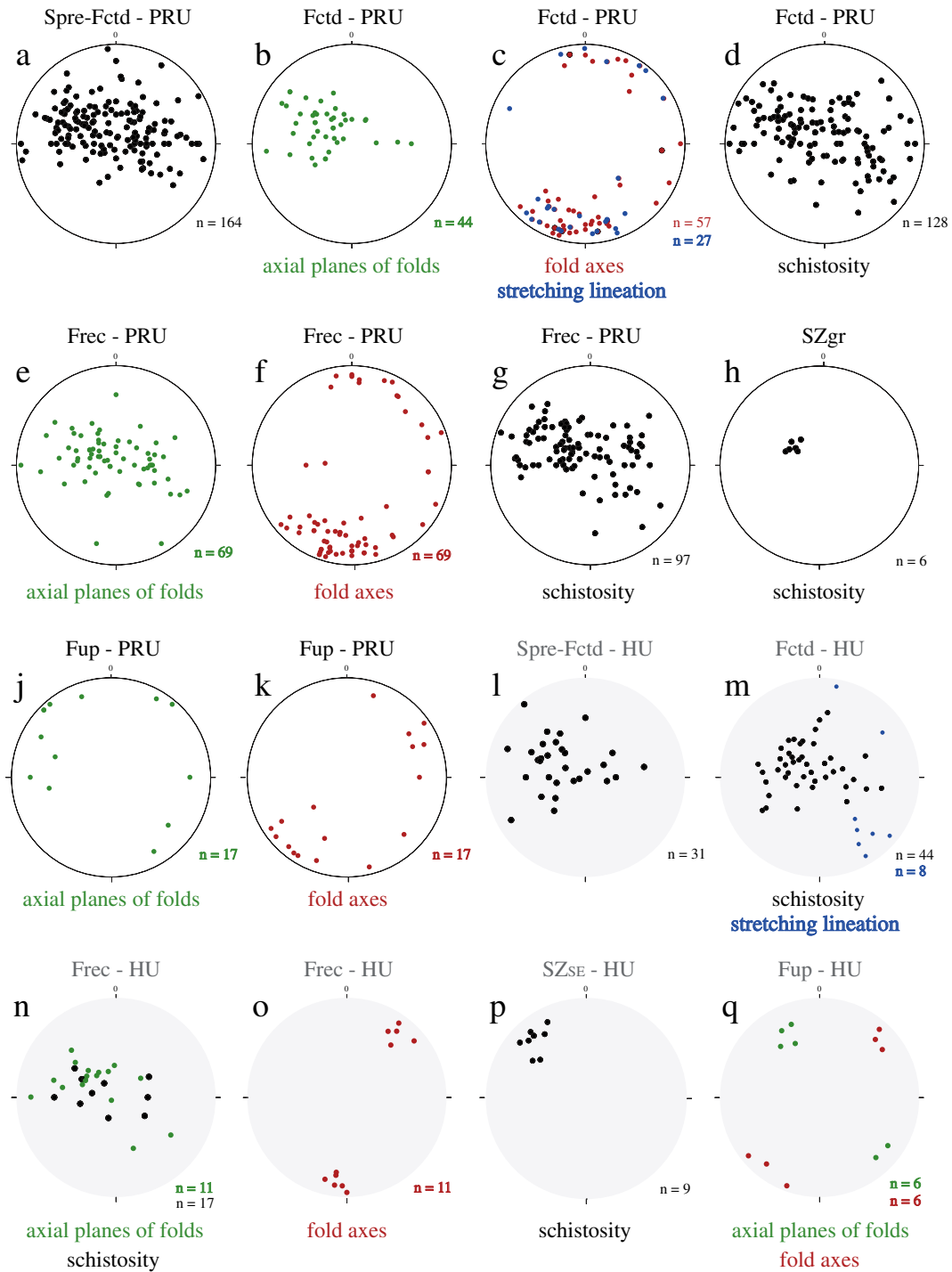
Fig. 10. Lower hemisphere Schmidt projection plots of structural elements in the study area (see explanation in the text). PRU = Punta Rossa Unit; HU = Hermite Unit.
