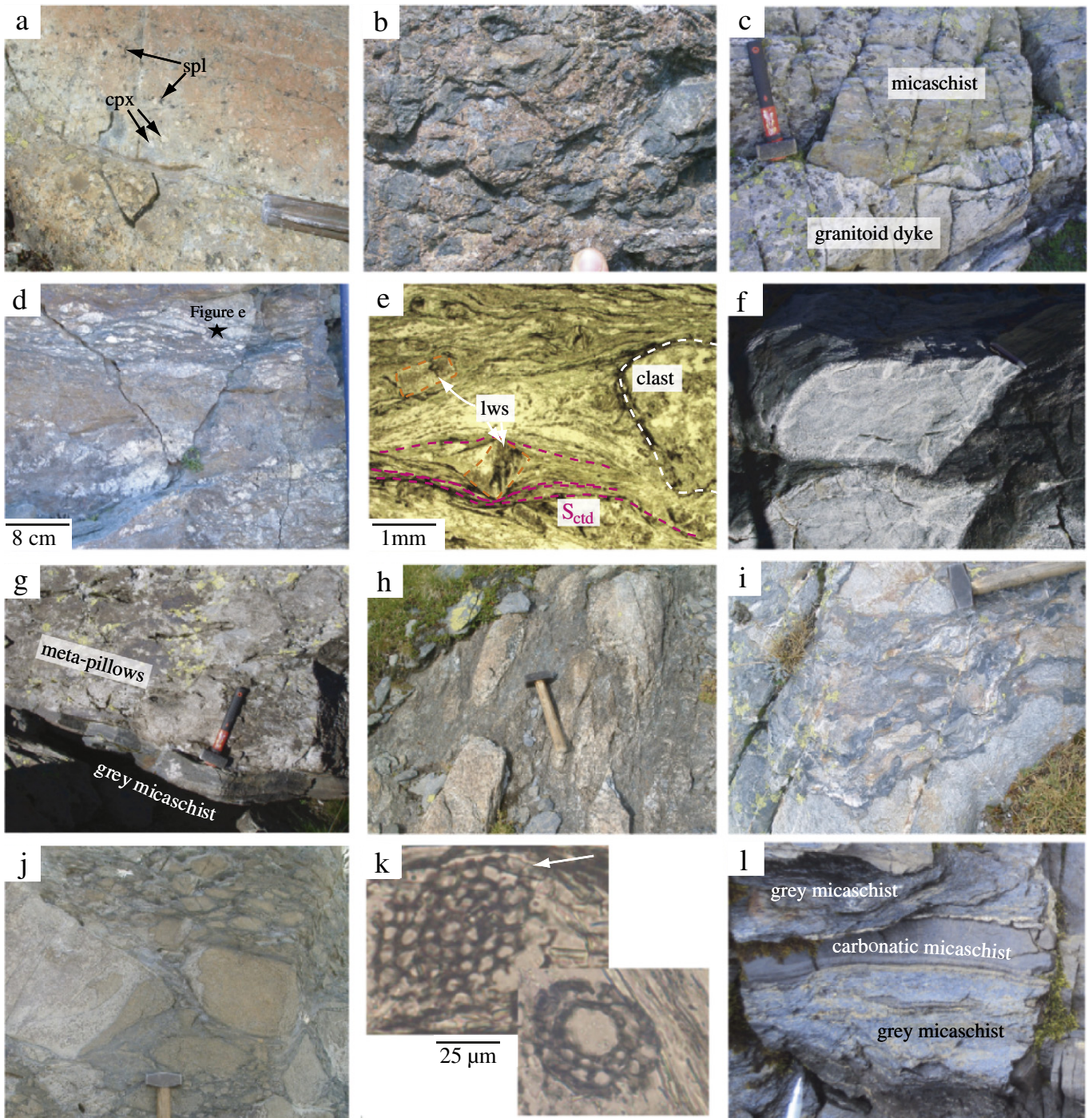
Fig. 5. Lithostratigraphic composition of the Punta Rossa unit: (a) serpentinized ultramafics with textural relicts of the peridotite clinopyroxene and spinel; (b) clast-supported ultramafic breccia at the contact with metamorphic polygenic breccia; (c) metagranitoid dyke intrusive into black micaschists in Paleozoic basement; (d) metamorphic fault breccia developed at the expense of a Paleozoic granitoid; (e) polymineralic clasts are wrapped around by a chlorite + white mica metamorphic fabric, which post-dates crystallization of lawsonite, now replaced by white mica and epidote. These observations indicate that Alpine metamorphism post-dated brittle fracturing; (f) meta-pillow; (g) overturned contact between meta-pillows and gray micaschists; (h, i, j) different types of sedimentary breccia, with ultramafic clasts (h), metagabbro, micaschist and granitoids clasts (i) and with clasts of metagabbros with ophitic texture (j); (k) microfossils preserved in the gray micaschists. Arrow indicates a chloritoid crystal; (l) transition between micaschist and carbonate micaschist.
