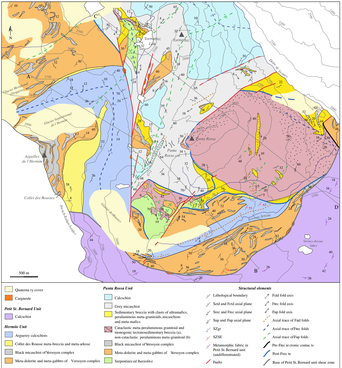
Fig. 3. Geological map of the area surrounding the Punta Rossa peak, with structural elements classified based on field relationships and microstructural observations (see text for details).
