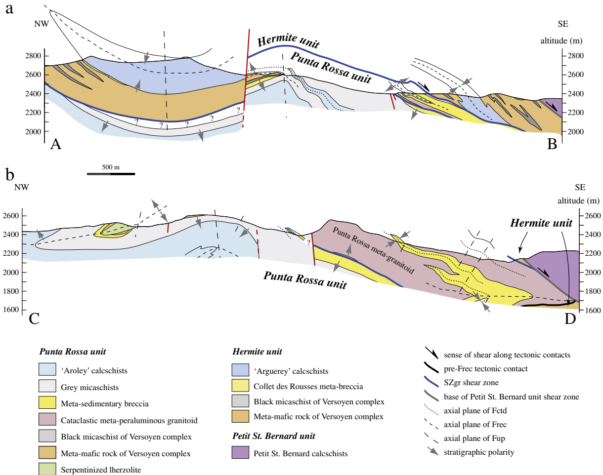
Fig. 9. Cross sections of the study area. Note that in the NW part of the AB section the lithological composition of the Punta Rossa unit directly underneath the Hermite unit has been omitted. This approach is justified by uncertainties in projecting ultramafics, Paleozoic basement and meta-breccia, due to the marked pre-Alpine lateral heterogeneities.
