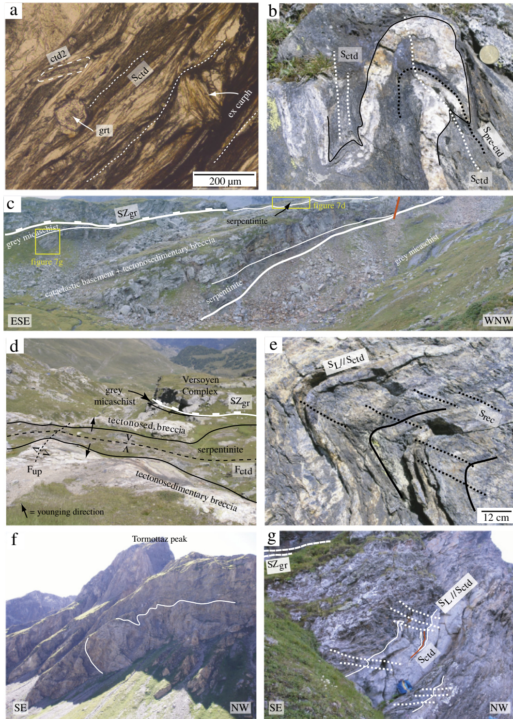
Fig. 7. Structural elements of the Punta Rossa unit. The oldest folds commonly recognizable in the field ( F_{ctd} ) develop a tightly spaced axial planar cleavage (a; S_{ctd} ) and locally deform pre-existing folds (b; F_{pre-S_{ctd}} ). Pre- S_{ctd} metamorphism is indicated by former carpholite porphyroclasts, now replaced by chlorite + white mica. Note that S_{ctd} is not deflected around garnet and chloritoid 2 porphyroblasts, indicating that their crystallization post-dated F_{ctd} . (c, d) Ultramafics and metagranitoids to the south of Punta Rossa crop out in the core of F_{ctd} synforms, with the upper limb preserving a normal stratigraphic polarity, with tectonosedimentary breccias and gray micaschist overlying serpentinites and Paleozoic basement. (e) Hinge area of a F_{rec} fold, with the characteristic spaced axial planar cleavage; (f) large scale F_{rec} fold on the NE side of Tormottaz peak. Note the contact between gray micaschists and calcschists steepening up in the proximity of the mountain top as a result of F_{up} . (g) The Punta Rossa unit is bounded upward by an extensional shear zone ( SZ_{gr} ). Top-to-the-SE sense of shear is defined based on the asymmetry of folds affecting F_{ctd} in the immediate footwall of the contact (f). Note that shear zones related to SZ_{gr} also run at the bottom of the cliff in the foreground in (c), where ultramafics are directly underlain by gray micaschists without the presence of tectonosedimentary breccia.
