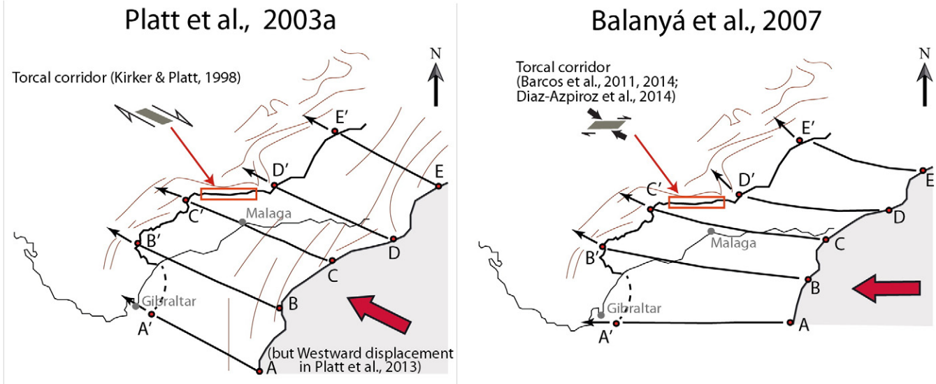
Fig. 3. Displacement of the Alboran Domain with respect to the fold and thrust belt of the Western Subbetics and Betic Flysch Trough, as proposed by Platt et al. (2003a) and Balanyá et al. (2007). Initial contour of the Alboran Domain from Kirker and Platt (1998).
