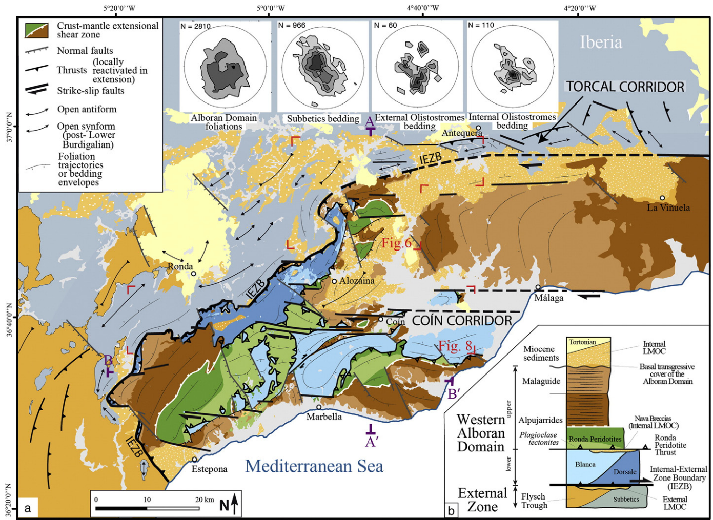
Fig. 4. (a) Simplified structural map of the Western Betics (redrawn after IGME ( http://info.igme.es/cartografia/magna50.asp?c=s ) and our own mapping) with location of the cross-sections AA' and BB' of Fig. 5. (b) General vertical section, showing the two main tectonic contact (IEZB and Ronda Peridotites Thrust) and the main tectonic units, from bottom to top: Subbetics and Flysch through unit, Blanca and Dorsale, Ronda Peridotites, Alpujarride, Malaguide, Internal and External LMOC and Tortonian sediments. Red marks: location of Figs. 6 and 8. Stereoplots of the foliation in the Alboran domain (2810 measurements) and of the bedding in the Subbetics, External and Internal Olistostromes (1136 measurements) are shown in the top of the figure.
