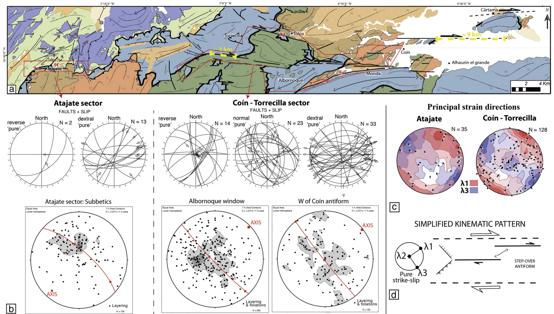
Fig. 8. (a) Structural map of the Coín corridor (lithotypes after personal observations; Chamón Cobos et al., 1972; Del Olmo Sanz et al., 1984, 1990; Mazzoli et al., 2013; Moreno Serrano et al., 1991; Piles Mateo et al., 1972a, 1972b). Symbols are the same as in Fig. 6 (see synthetic vertical section in Fig. 6a). Red numbers indicate the location of Fig. 9 photographs. Paleomagnetic declinations for the Subbetics are drawn after Platzman and Lowrie (1992), Villalain et al. (1994) and Kirker and Platt (1998) (see Fig. 6a for the symbols). The displacement along the strike-slip faults in key areas is marked in yellow. (b) Stereoplots of data collected in the areas marked in red in Fig. 8a and (c) principal strain directions. For (b) and (c) same technical specifications than in Figs. 6b and c. (d) Simplified kinematic pattern of the Coín corridor with branch-type termination and relay structures between left-stepping segments of the deformation zone. Figure S2 in supplementary material presents a complete description of the principal strain directions.
