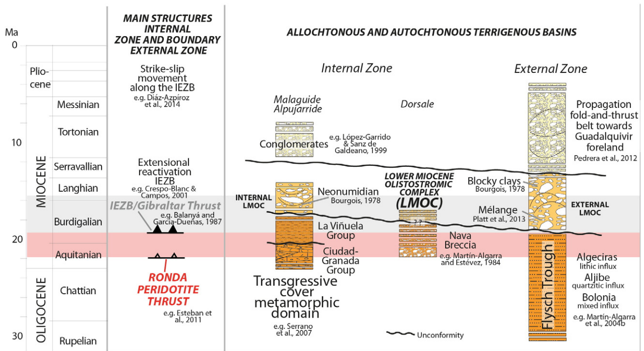
Fig. 2. The main Miocene tectonic events of the Western Betics (after Crespo-Blanc and Campos (2001); Díaz-Azpiroz et al. (2014); Esteban et al. (2011) and Kirker and Platt (1998)) and the Lower Miocene deposits (after López-Garrido and Sanz de Galdeano (1999); Martín-Algarra et al. (2004a, 2004b); Martín-Algarra and Vera (2004); Pedrera et al. (2012); Serrano et al. (2007)).
