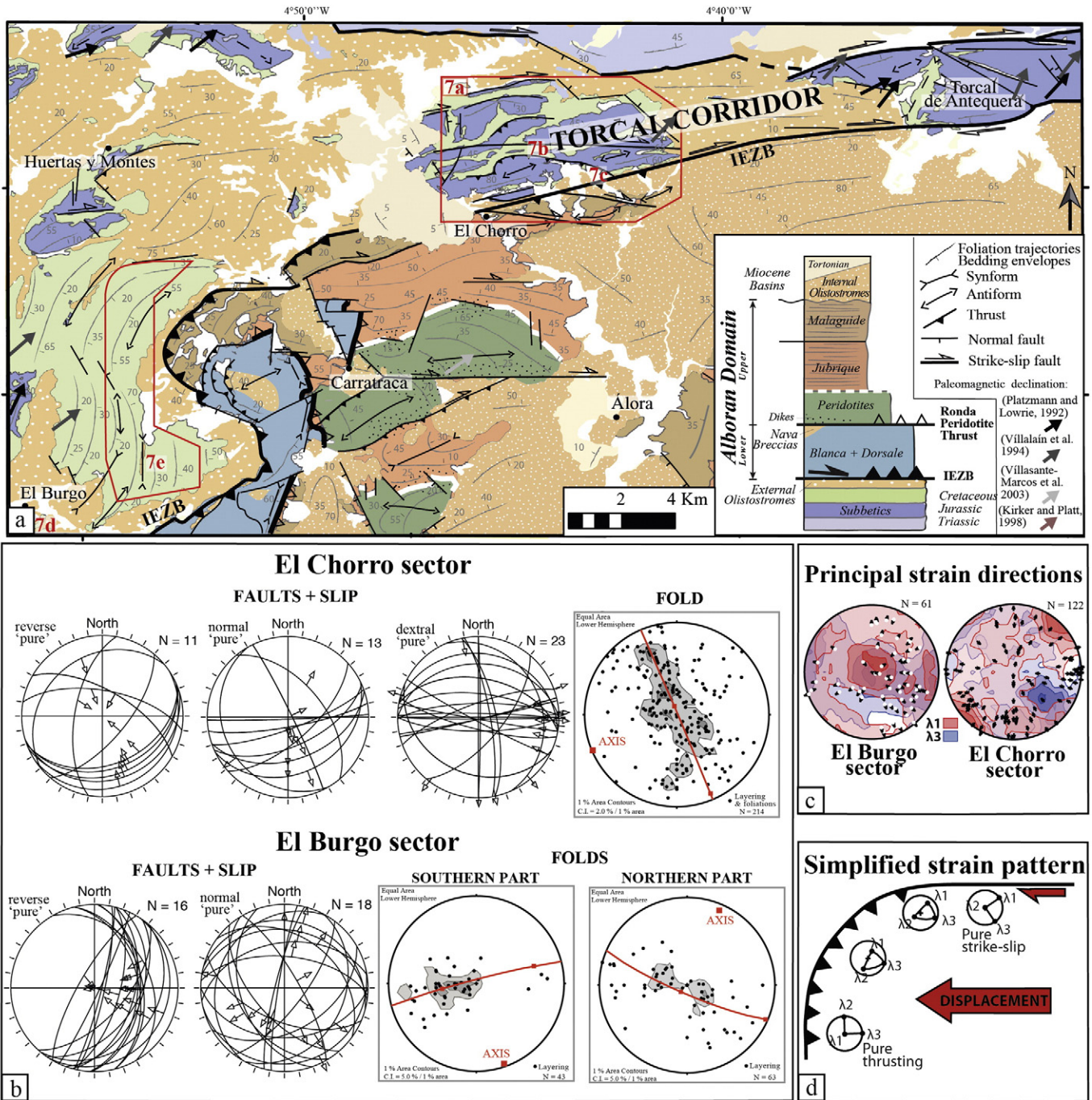
Fig. 6. (a) Structural map of the Torcal corridor between El Burgo and the Torcal de Antequera (lithotypes after our own mapping and previous works (Argles et al., 1999; Barcos et al., 2011; Cano Medina, 1990; Chamón Cobos et al., 1972; Cruz San Julian, 1990; Del Olmo Sanz et al., 1990). A synthetic vertical section shows the main tectonic units and contacts. Red numbers indicate the location of Fig. 7 photographs. Paleomagnetic declination for the Subbetics and for the Alboran Domain are drawn after Platzman and Lowrie (1992), Villalaín et al. (1994) and Villasante-Marcos et al. (2003). (b) Stereoplots of data collected in the areas marked in red on the map of Fig. 6a (lower hemisphere; Schmidt net; using OSXStereonet: version 9.2.0. http://www.uix.us.no/~nestor/work/programs.html and Fsa: Fault slip analysis software. Version 35.1. http://www.pages-perso-bernardcelierier.univmontp2.fr/software/dcm/fsa/fsa.html ). Faults with an oblique slip-vector (higher than 20° from the ideal pure-slip vector for each fault) are not reported; (c) Principal strain directions obtained with FaultKin ( http://www.geo.cornell.edu/geology/faculty/RWA/programs/faultkin.html ). For the sake of clarity, only striae and slip directions are indicated with the contours of λ1 (red) and λ3 (blue) distribution obtained for each fault mirror measured. For a detailed strain analysis of the corridor see supplementary material . (d) Simplified evolution of the principal strain directions from frontal to lateral ramps of Fig. 6a. Red arrow: displacement of the Alboran Domain. Figure S1 in supplementary material presents a complete description of the principal strain directions.
