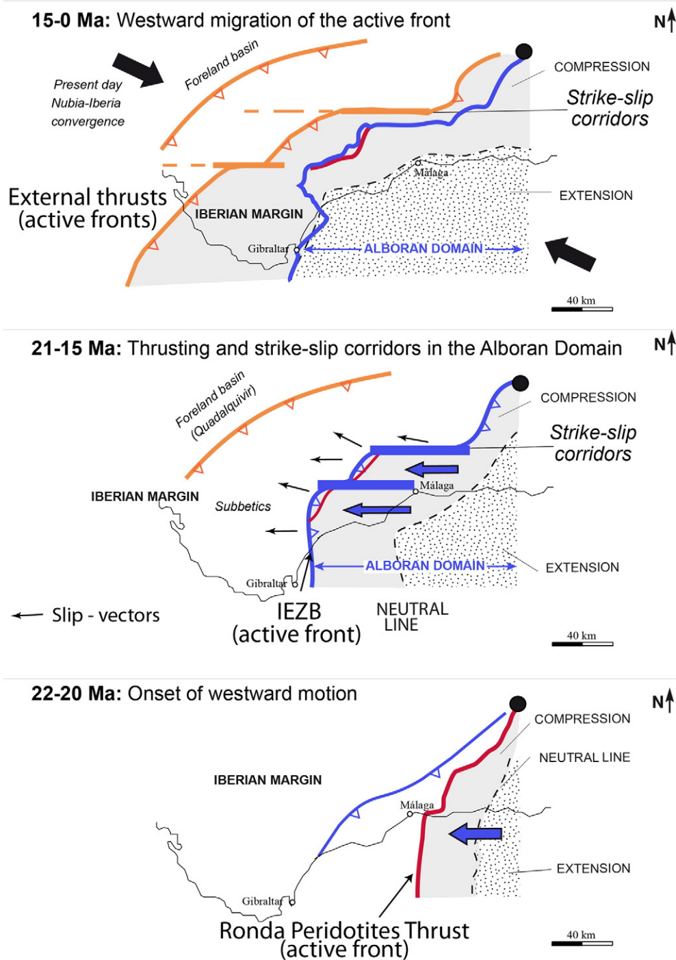
Fig. 10. Three-stage sketch of the westward displacement of the Alboran Domain from Lower Miocene to present day the progressive development of thrusts and strike-slip corridors. A thick line marks the Active front and domains sustaining compression or extension are respectively in white or dotted-white. The three successive stages are from bottom to top 1) Onset of westward motion (22–20 Ma) marked by the Ronda peridotites thrust (thick red line), 2) westward motion of the Alboran domain (22–15 Ma) mainly accommodated by the IEZB (thick blue line) and strike slip corridors (blue E-W bands), 3) westward migration of the active front in the External Zone (15–0 Ma, thick orange line), leading to an extensional reactivation (dotted domain) of the Alboran domain. Black arrows: Present-day Nubia–Iberia direction of convergence in the northern part of the Gibraltar arc (from Vernant et al., 2010).
