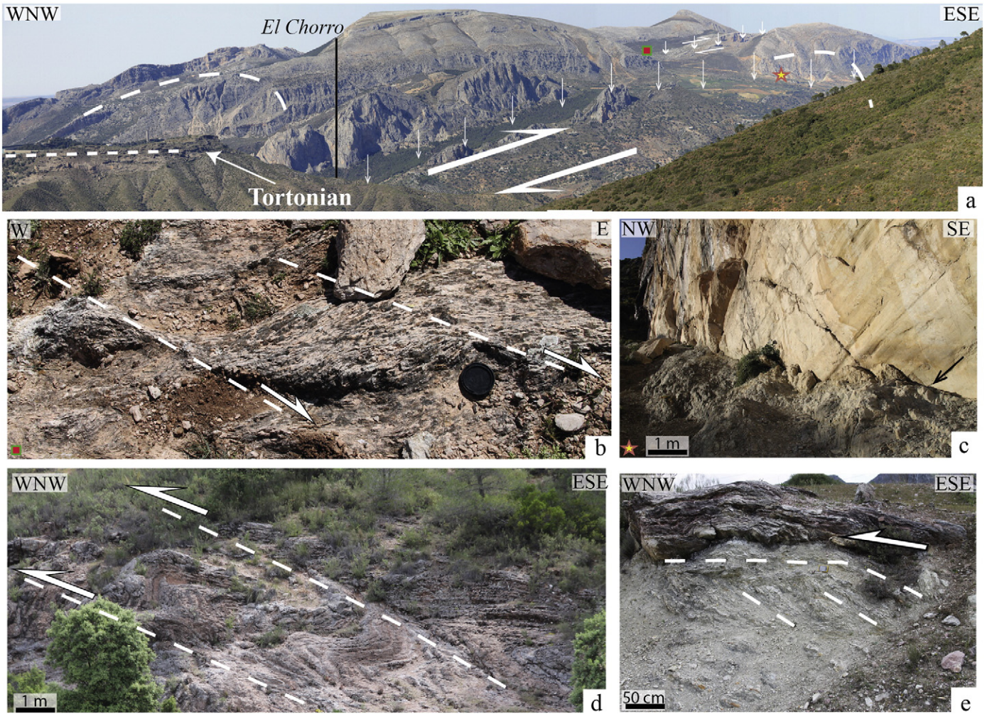
Fig. 7. Some typical structures of the El Chorro sector (see location in Fig. 6a): (a) Panoramic view of the Torcal strike-slip deformation zone and of the anticline NE of El Chorro village. Note the flat-lying Tortonian on the left-side. Square and star indicate the location of Fig. 7b and c, respectively. (b) Riedel-type shear planes indicating a dextral slip in an E-W vertical fault zone inside Upper Cretaceous marly-limestones. (c) Normal fault with a strong oblique dextral-slip component at the contact between Jurassic limestones and Cretaceous marly-limestones. (d) Fault-propagation-folds and (e) a flat-and-ramp structure, show a top-to-the-WNW sense of shear in the Upper Cretaceous marly-limestone close to El Burgo.
