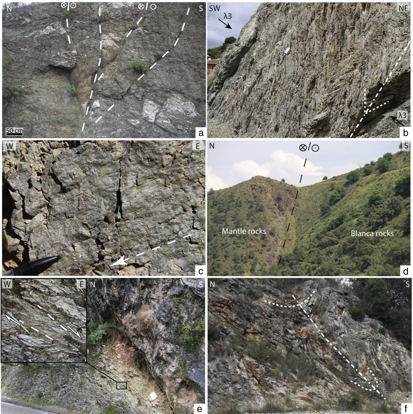
Fig. 9. Some typical structures of the region between Coín and Torrecilla (see locations in Fig. 8): (a) Negative flower structures in a right-slip fault-zone with slip-vectors gently plunging to the E. (b) En-échelon chevron folds without axial-plane cleavage and axes gently plunging to the ENE. (c) Wear striae, plough marks and intersections with Riedel-shear plane on an E-W vertical fault mirror. (d) Panoramic view of a vertical WNW-ESE dextral strike-slip fault, cross-cutting the Ronda Peridotites and “Blanca” migmatites. Some typical structures of the strike-slip segment of the IEZB nearby Atajate: (e) Dextral strike-slip fault zone between “dorsalian” Jurassic massive limestones and Cretaceous marly limestones with an oblique slip-vector and (f) E-W trending fold inside Cretaceous layered limestones.
