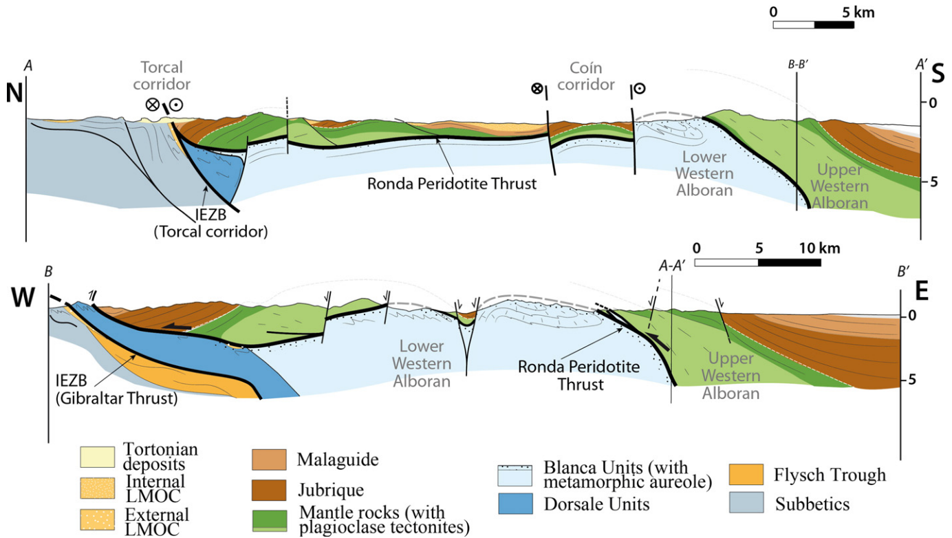
Fig. 5. Synthetic cross-sections (see location in Fig. 4). Interpretation below 5 km is omitted due to the lack of geophysical data.
