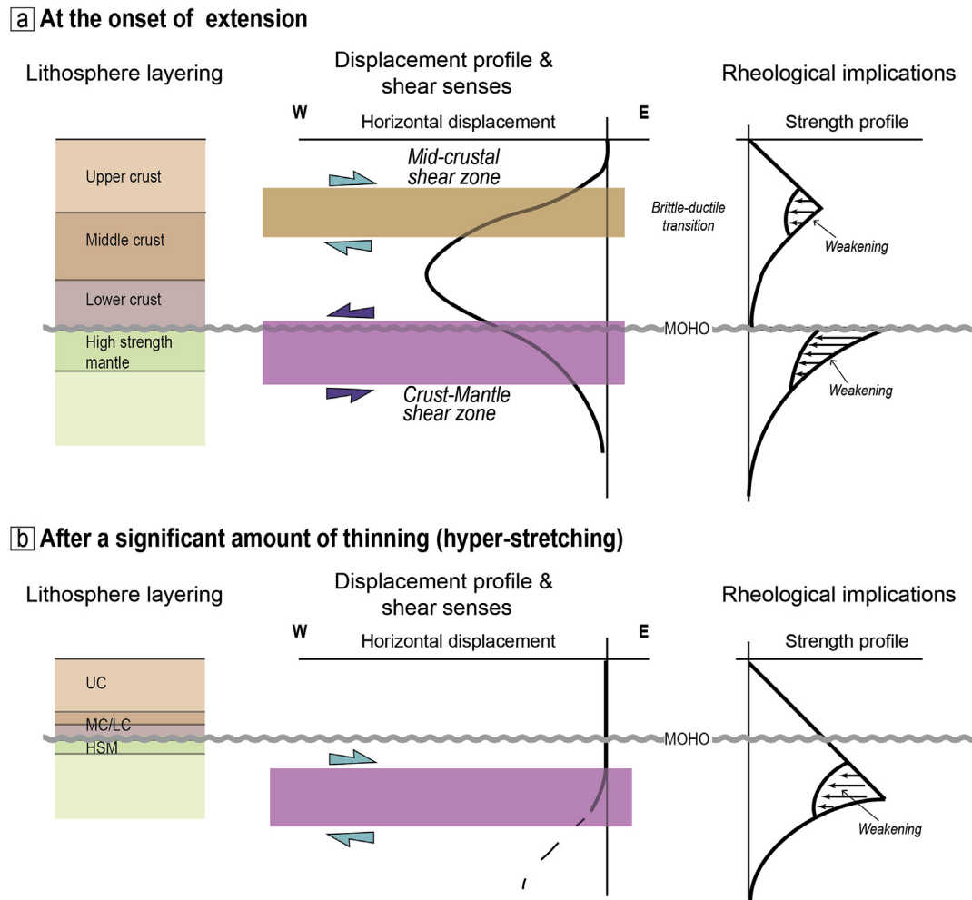
Fig. 9. Summary of shear sense variations with depth and their implications in terms of horizontal displacement and rheology (strength profile), (a) at the onset of extension and (b) after a strong crustal thinning in the hyper-stretched portion of the lithosphere.
