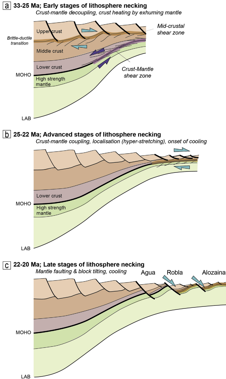
Fig. 10. Three-stage conceptual model of lithosphere necking summarizing the progressive deformation recorded in the crust and mantle units of the Carratraca area. (a) Early stages controlled by the mid-crustal shear zone and the crust-mantle shear zone with opposite senses of shear. (b) Advanced stages characterized by localization of stretching at rift center leading to an extreme thinning of the ductile crust and omission of the lower crust. (c) Late stages of high-angle faulting cutting through the strongly attenuated crust and the cooling mantle.
