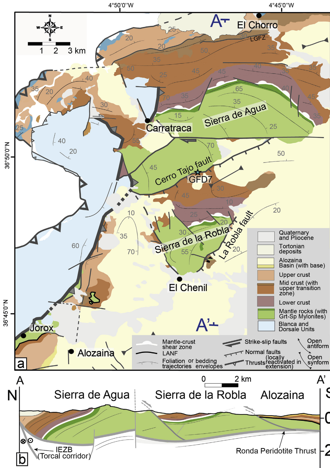
Fig. 3. (a) Structural map of the Carratraca peridotitic massives (synthesized after Chamón Cobos et al., 1972; Cano Medina and Ruiz Reig, 1990; Cruz San Julián, 1990; Del Olmo Sanz et al., 1990; Soto and Gervilla, 1991; Argles et al., 1999; Tubía et al., 2004 and Frasca et al., 2015). Green star: position of the sample (GFD7) collected for the ^{40}\text{Ar}/^{39}\text{Ar} dating. IEZB: Internal-External Zone Boundary; LANF: Low angle normal Fault; LGFZ: Los Grenadillos Fault Zone. (b) NS cross-section showing the geometry of the three blocks of Sierra de Agua, Sierra de la Robla and Alosaina. See location in (a). (For interpretation of the references to colour in this figure legend, the reader is referred to the web version of this article.)
