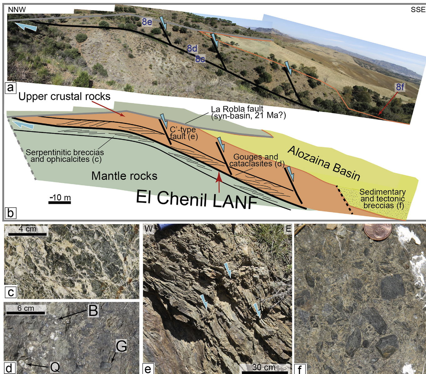
Fig. 8. Low-angle normal fault (LANF) in the hyper-stretched portion of the rift (El Chenil area; see location in Fig. 6). (a) Landscape view of the El Chenil LNF. (b) Geological interpretation of the El Chenil fault zone (for detailed map and measurements see Fig. S2). (c) Photograph of ophicalcite. (d) Fault gouge in the fault core zone with clasts of quartzveins (Q), breccia (B) and gneiss (G). (e) C'-type shear bands (shown by blue arrows) in the upper crustal rocks indicating a top-to-E sense of shear. (f) Sedimentary breccia at the base of the Alozaina basin with clasts of upper crustal rocks. (For interpretation of the references to colour in this figure legend, the reader is referred to the web version of this article.)
