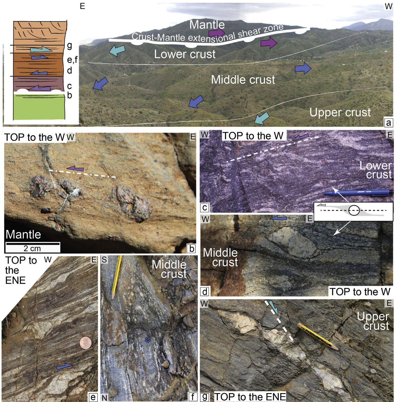
Fig. 5. Types of shear indicators used in crust and mantle rocks (a) Landscape view (from point 5a in Fig. 4) of the thinned lithosphere in the Sierra de Agua. Left inset: Summary of senses of shear at the different lithosphere levels (not to scale; green: mantle; violet: lower crust; dark brown: middle crust; light brown: upper crust) with location of photographs (see location in Fig. 4). (b) Top-to-W sense of shear in the mantle: deflection of a pyroxenite layer in the Grt-Sp mylonitic foliation. (c) Top-to-W sense of shear in the lower crust: melt in veins and in pressure shadows around a garnet porphyroclasts and C'-type shear-bands, locally enriched in melt, in molten granulites. (d) Top-to-W sense of shear in the middle crust: sigmoidal stretched leucosome. (e) Top-to-E sense of shear in the middle crust: sigmoidal stretched leucosome. (f) Eyed-type section of a sheath fold in the middle crust in the sillimanite gneisses. (g) Top-to-E sense of shear in the middle/upper crust: C'-type brittle-ductile shear bands in the andalusite schists. (For interpretation of the references to colour in this figure legend, the reader is referred to the web version of this article.)
