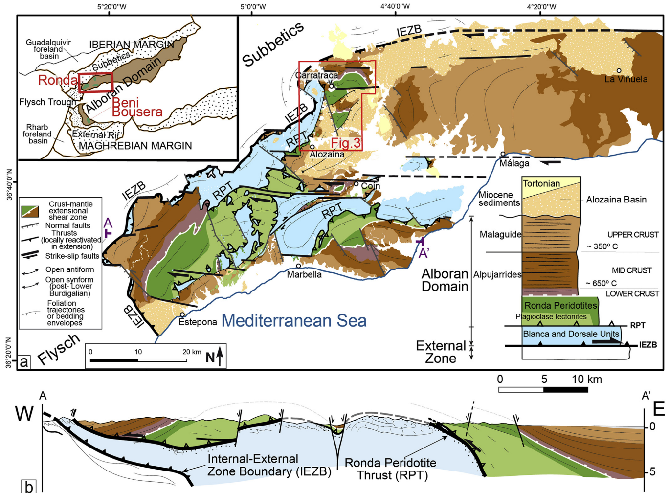
Fig. 1. a) Tectonic map of the Western Betics with foliation trajectories (modified after Frasca et al., 2015) showing the main geological units: Ronda peridotites with plagioclase tectonites (dark green and pale green), lower, middle and upper crustal rocks above the peridotites (violet, dark brown and pale brown), crustal rocks below the peridotites (pale blue), lower Miocene Alosaina basin (beige) and Tortonian basins (pale yellow). Major tectonic contacts: Ronda Peridotites Thrust (RPT), Internal-External Zone Boundary (IEZB), crust-mantle extensional shear zone (white line). Top left inset: Location of the study area in the Betic-Rif belt with the location of the Ronda-Beni Bousera mantle bodies. Bottom right inset: synthetic vertical section of the lithological and tectonic units of the Western Betics. b) E-W trending cross-section; see location AA' in (a). (For interpretation of the references to colour in this figure legend, the reader is referred to the web version of this article.)
