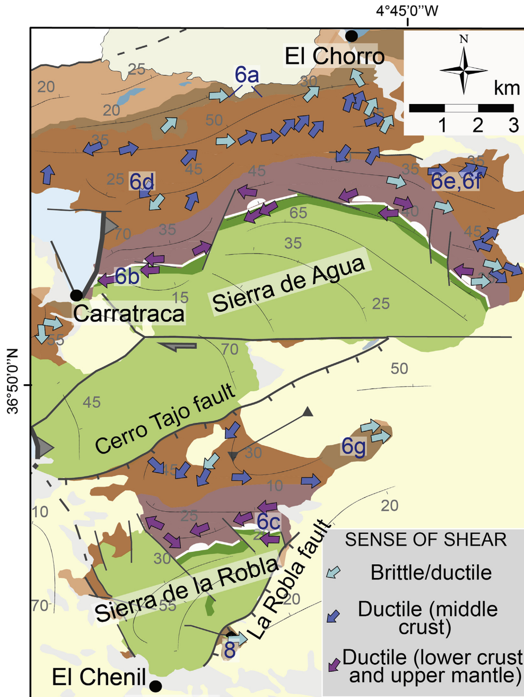
Fig. 6. Map of mean senses of shear in the Carratraca area. Colors of geological units like in Fig. 3. Ductile shear in the mantle and lower crust (Violet arrows) and in the middle crust (Blue arrows). Brittle/ductile shear, mainly observed in the upper crust (Pale blue) (For the whole set of lineation and shear criteria see “supplementary material”, Fig. S1). (For interpretation of the references to colour in this figure legend, the reader is referred to the web version of this article.)
