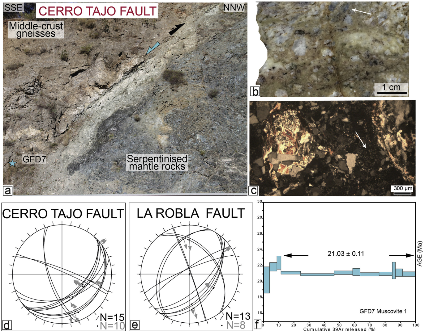
Fig. 4. Kinematics and age of high-angle normal faults. (a) Outcrop photograph of the Cerro Tajo fault that put in contact middle crust gneisses with serpentinitised mantle rocks (b) Hand-specimen (GFD7) of the fault breccia sampled for ^{40}\text{Ar}/^{39}\text{Ar} dating (see location in Fig. 3a). White arrow: clast of the gneiss protolith containing only biotite. (c) Thin-section of sample GFD7 showing the formation of white mica pseudomorph after garnet. White arrow: very small white micas in the matrix (for details see “supplementary material”, Fig. S3). (d and e) Stereoplots of fault surfaces (lower hemisphere projection on a Schmidt net; FSA software by Célérier, 2013; version 35.2) for Cerro Tajo fault and La Robla fault (e) (see location of the faults in Fig. 3a). Great circles: fault planes. Grey arrows: direction of motion on fault surfaces. (f) ^{40}\text{Ar}/^{39}\text{Ar} age spectrum for the mm-sized white micas extracted from the sample GFD7 (see method and analytical data in “supplementary material”).
