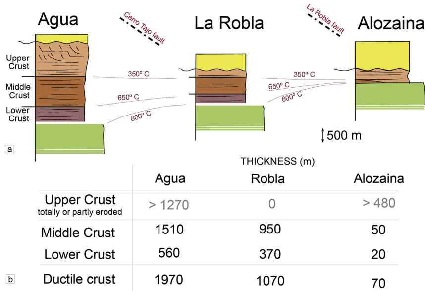
Fig. 7. Variations in crustal thickness. (a) Crustal thickness estimates in the Agua, La Robla and Alozaina blocks (green: mantle; violet: lower crust; dark brown: middle crust; light brown: upper crust) (See location in Fig. 3). (b) Estimates of the average thickness of the upper, middle and lower crust in the three blocks, made from local cross-sections that take into account variations in mean foliation dip. (For interpretation of the references to colour in this figure legend, the reader is referred to the web version of this article.)
