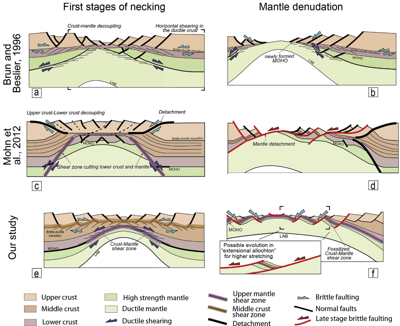
Fig. 11. Comparison of models of lithosphere necking up to mantle exhumation, which evolve either dominantly symmetrical (a and b) or asymmetrical (c and d), with the lithosphere-scale deformation pattern documented in the western Betics (e and f) (as summarized in Figs. 9 and 10).
