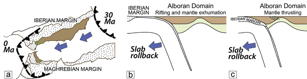
Fig. 2. (a) Subduction slab rollback setting of the Ronda peridotites in the Alboran domain, showing the present day geometry of the trench and its hypothetical position at 30 Ma. (b) Rifting at the front of the subduction upper plate responsible for mantle exhumation. (c) Rift inversion and thrust emplacement of the Ronda Peridotites on top of the Iberian margin (modified after Précigout et al., 2013).
